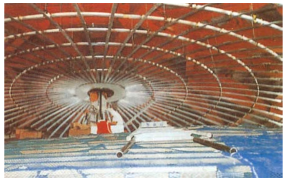
Dome Ceiling Suspension System
